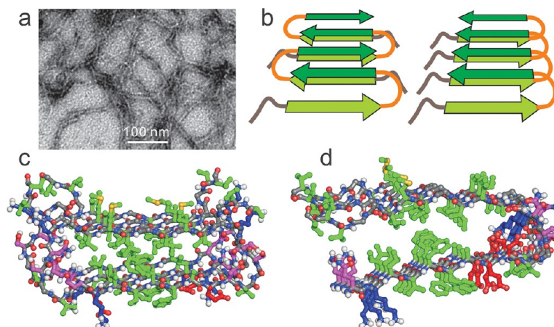
FIGURE 4. (a) Negatively stained TEM image of D23N- A\beta_{1-40} fibrils, prepared by a method that selects metastable, antiparallel \beta -sheet structures. 13 (b) Schematic comparison of antiparallel (left) and parallel (right) cross- \beta structures that can be constructed from similar U-shaped peptides. (c) Structural model for metastable D23N- A\beta_{1-40} fibrils developed from solid state NMR data, 13 viewed in cross section. Two repeats (four D23N- A\beta_{1-40} chains, residues 15–40 only) are shown, with side chains colored as in Figure 2. (d) Residues 15–40 of one cross- \beta unit within a 2-fold A\beta_{1-40} fibril. Comparison with panel (c) shows how similar sets of hydrophobic interactions in the core of the cross- \beta unit can stabilize both parallel and antiparallel structures.
