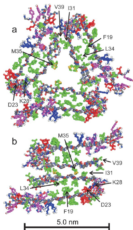
FIGURE 2. Structural models for A\beta_{1-40} fibrils developed from solid state NMR and electron microscopy data. 2,3 Models with 3-fold (a) and 2-fold (b) symmetry correspond to "twisted" fibrils and to individual filaments within "striated ribbon" fibrils in Figure 1a and b, respectively. Models include residues 9–40 and are viewed in cross section, with the long fibril axis perpendicular to the page. Four repeats of the parallel cross- \beta structures are shown, with side chains of hydrophobic residues in green, polar residues in magenta, negatively charged residues in red, and positively charged residues in blue.
