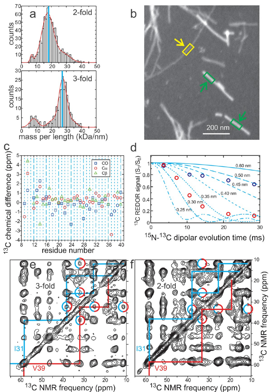
FIGURE 3. Examples of experimental data that lead to the structural models for A\beta_{1-40} fibrils in Figure 2. (a) Mass-per-length (MPL) histograms derived from dark-field transmission electron microscopy, 19 showing the predominant values of 18 and 27 kDa/nm expected for 2-fold and 3-fold symmetric cross- \beta structures. (b) Example of an unstained dark-field TEM image, showing a 3-fold A\beta_{1-40} fibril (yellow arrow) and tobacco mosaic virus particles (green arrows) that serve as MPL standards. Fibril MPL values are determined from the ratios of integrated intensities within yellow and green rectangles. (c) Differences in ^{13}\text{C} NMR chemical shifts between 2-fold and 3-fold A\beta_{1-40} fibrils, for backbone carbonyl, \alpha -carbon, and \beta -carbon sites. (d) Quantitative measurements of magnetic dipole-dipole couplings between K28 \zeta -nitrogen and D23 \gamma -carbon sites in 2-fold (red circles) and 3-fold (blue circles) fibrils, using a frequency-selective rotational echo double-resonance technique. 21 These data demonstrate the presence of D23-K28 salt bridge interactions in the 2-fold fibrils 3 and the absence of these interactions in 3-fold fibrils. 2 (e) Aliphatic region of a two-dimensional ^{13}\text{C} - ^{13}\text{C} NMR spectrum of 3-fold fibrils, prepared with uniform ^{13}\text{C} labeling of I31, G33, M35, G37, and V39, recorded with a 1.5 s mixing period that allows long-range crosspeaks to develop. Intraresidue crosspeaks for I31 and V39 are identified by cyan and red assignment paths, respectively. Cyan/red circles indicate inter-residue crosspeaks that imply proximity of I31 and V39 side chains, 2 as in Figure 2a. (f) Similar two-dimensional spectrum of 2-fold fibrils. Absence of clear crosspeaks in cyan/red circles implies a greater I31-V39 separation, as in Figure 2b.
